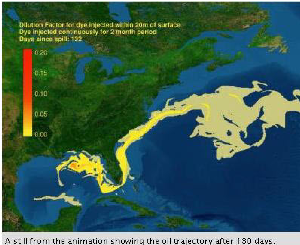
UCAR Model of oil slick movement after 130 days from original explosion
